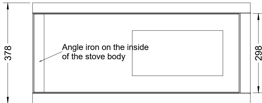
Bottom view with Angle Iron
