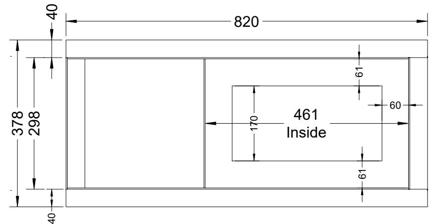
Top view with Angle Iron
